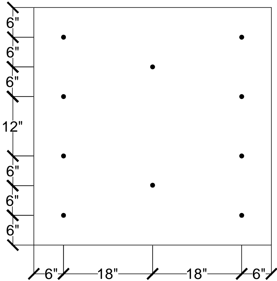
10 FASTENERS PER 4' x 4' BOARD
