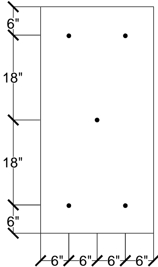
5 FASTENERS PER 2' x 4' BOARD
